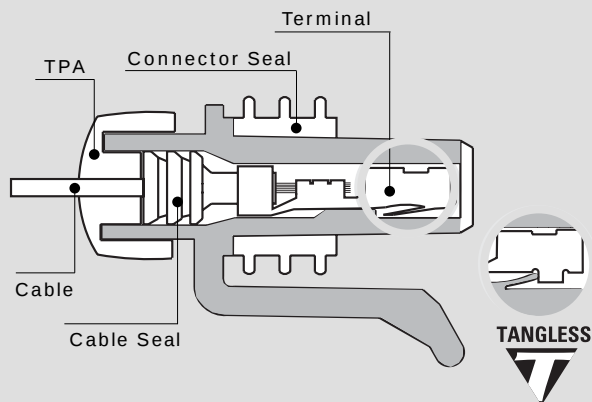
Female Connector Assembly
