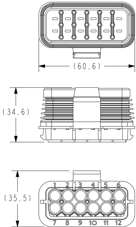
FRH-A12 HOUSING AND SEAL - PDM, FRH 12 POS (FOR TERMINALS AND SEALS SEE TABLE A)
