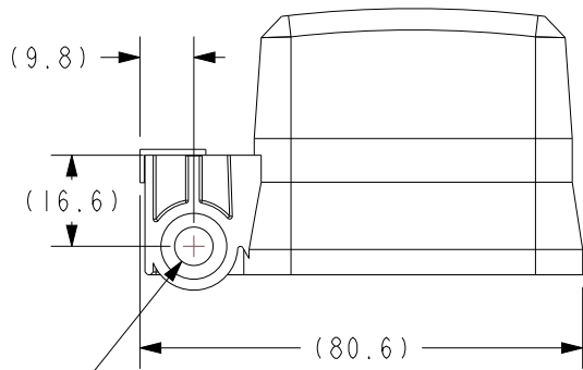
FRH-A12-CB-1 COVER - PDM, FRH 12 POS, SINGLE SIDE MOUNT, PLAIN
