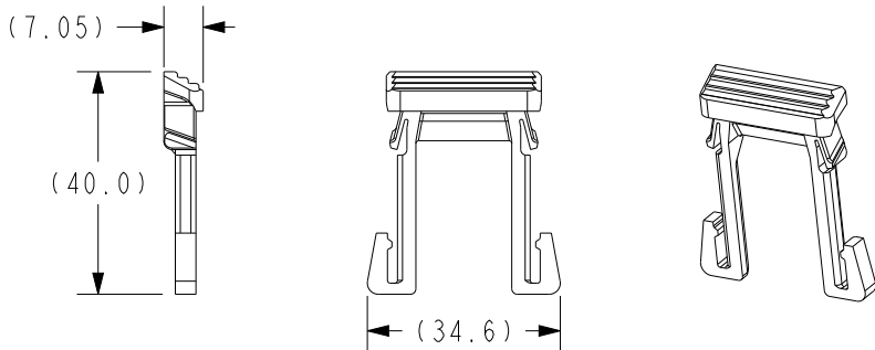
FRH-A-CPA CPA - PDM, FRH
