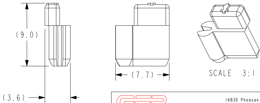
PDM-TK DIODE KEY
