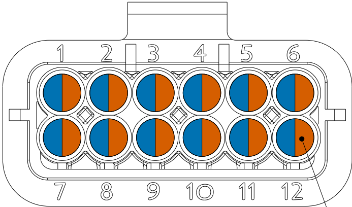
FRH-A12 HOUSING AND SEAL - PDM, FRH 12 POS
