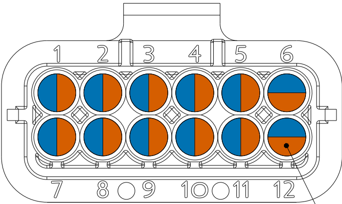
SC42-2018A-A001 HOUSING AND SEAL - PDM FRH 12 POS - ROTATED FUSE
