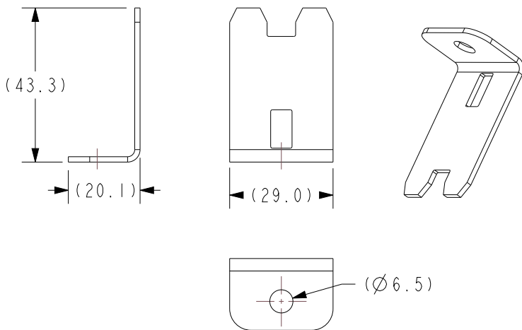
FRH-A12-MB-C1 BRACKET - PDM, FRH, 90° BENT, ZINC STEEL
