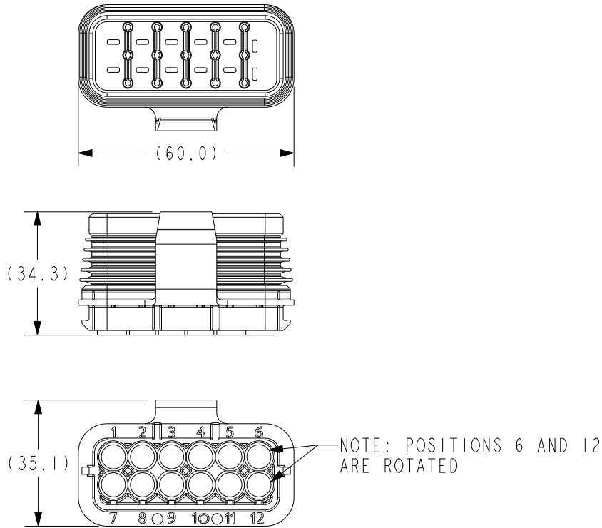
SC42-2018A-A001 HOUSING AND SEAL - PDM FRH 12 POS - ROTATED FUSE (FOR TERMINALS AND SEALS SEE TABLE A)
