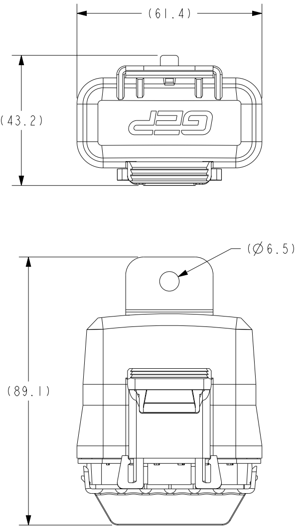
EXAMPLE CONFIGURATION WITH DIMENSIONAL INFO
